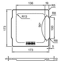
Cover (bamboe)
